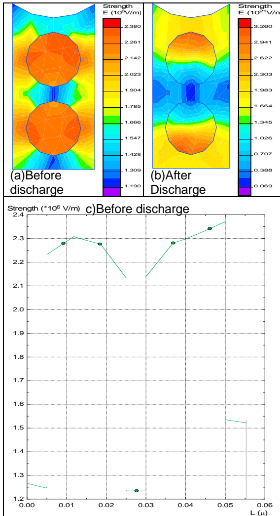
Figure 4.3: Electric field in Aerogel with curved electrode before and after Discharge
