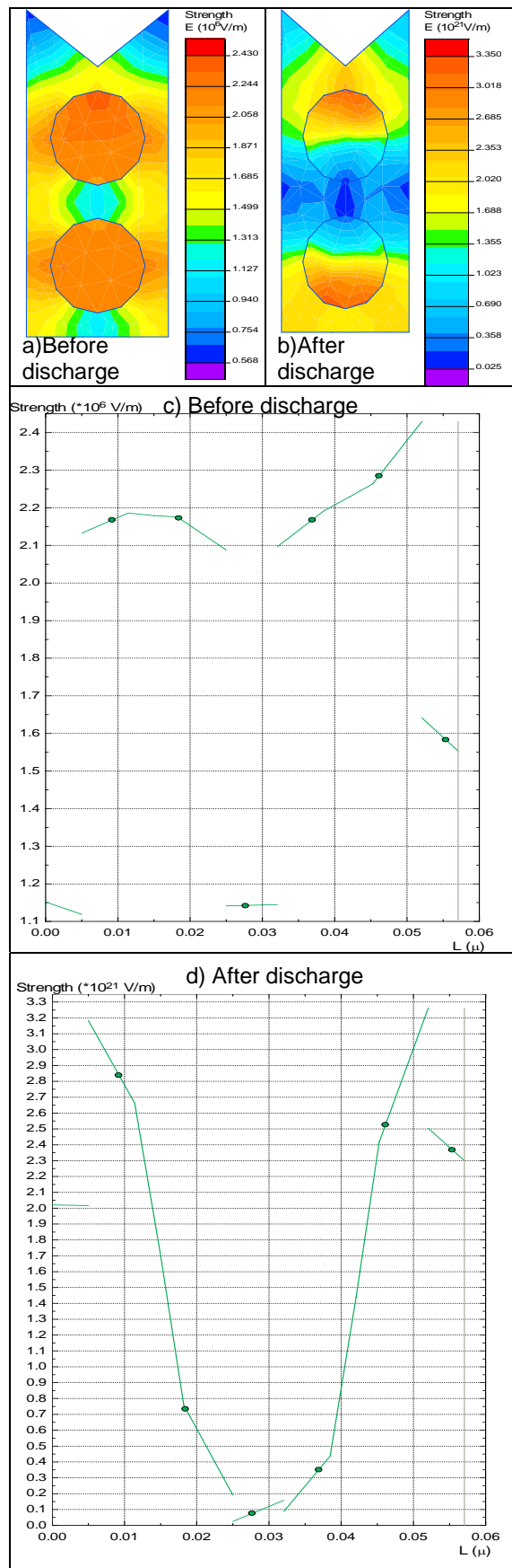
Figure 4.2: Electric field in Aerogel with pointed electrode before and after Discharge
