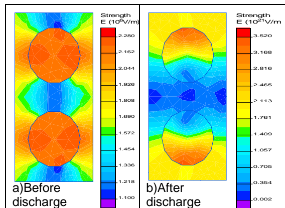
Figure 4.1-1: Electric field in Aerogel between flat electrodes before and after Discharge
