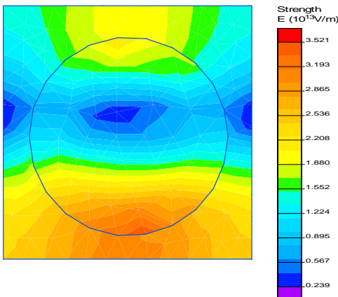
Figure 4: Electric field for a single isolated nanopore after Discharge
