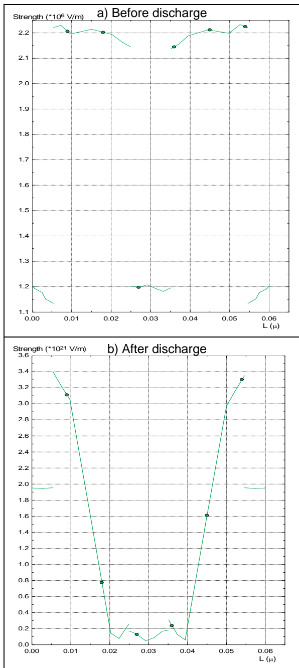
Figure 4.1-2: Electric field in Aerogel between flat electrodes before and after Discharge
