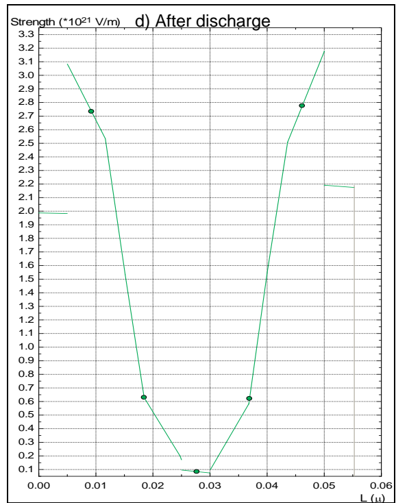
Figure 4.3: Electric field in Aerogel with curved electrode before and after Discharge
