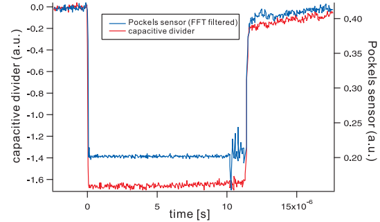
Figure 11: Steep-front square voltage measurement with digital filter.
