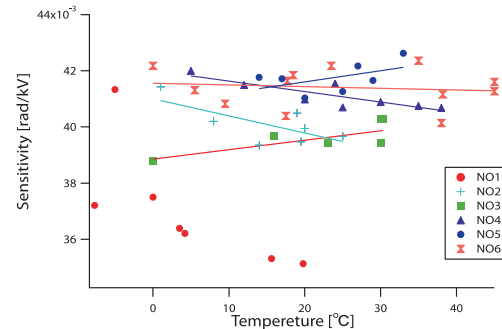
Figure 5: Sensitivity of BGO bars for 1300 nm light.
