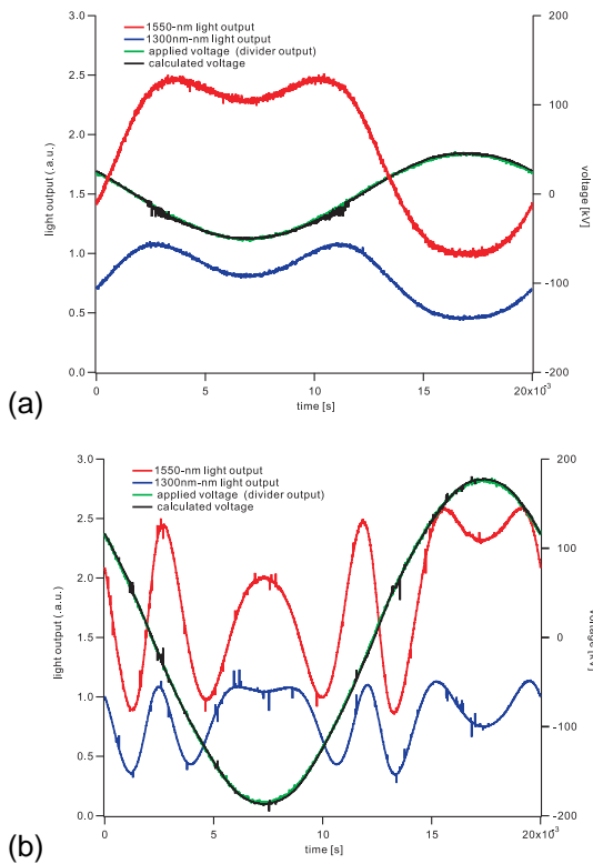
Figure 7: AC voltage measurement under (a) 50kV- and (b) 180kV- voltage application.
