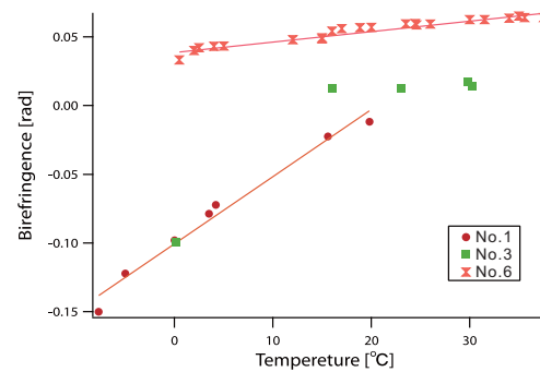
Figure 6: Natural birefringence of BGO bars for 1300 nm light.
