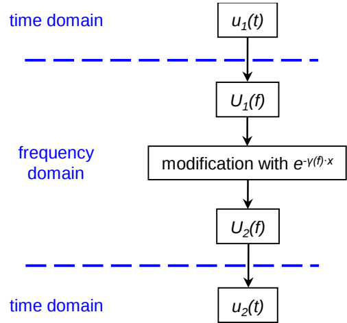
Figure 9: Main principle of frequency domain calculations.
